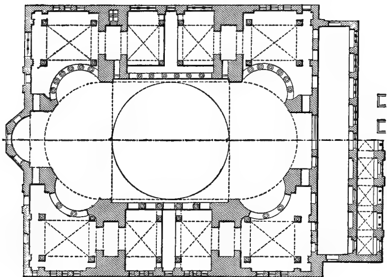
GROUND-PLAN OF THE CHURCH OF ST. SOPHIA
