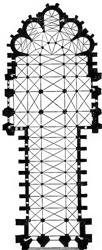
GROUND-PLAN OF RHEIMS CATHEDRAL
